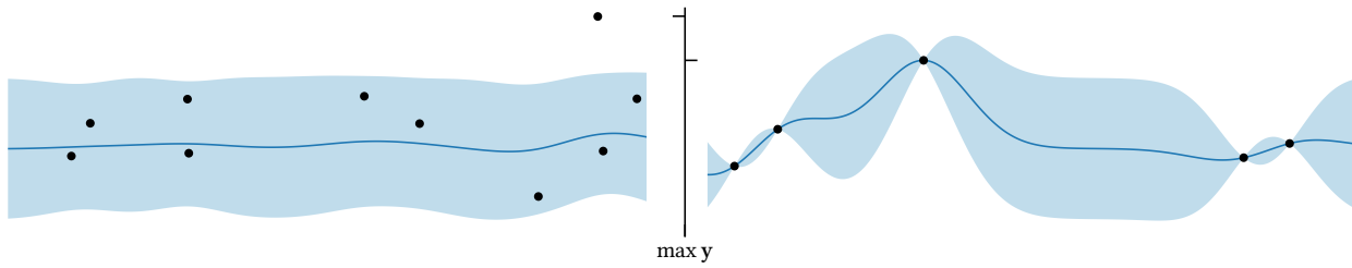
Figure 6.2: The utility u(\mathcal{D}) = \max y would prefer the excessively noisy dataset on the left to the less-noisy dataset on the right with smaller maximum value. The data on the left reveal little information about the objective function, and the maximum observed value is very likely to be an outlier, whereas the data on the right indicate reasonable progress.
