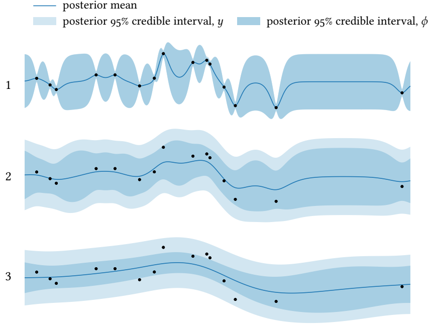
Figure 4.4: Posterior distributions given the observed data corresponding to the three settings of the model hyperparameters marked in Figure 4.3. Although remarkably different in their interpretations, each model represents an equally plausible explanation in the model posterior. Model 1 favors near-exact observations with a short length scale, and models 2–3 favor large observation noise with a range of length scales.
