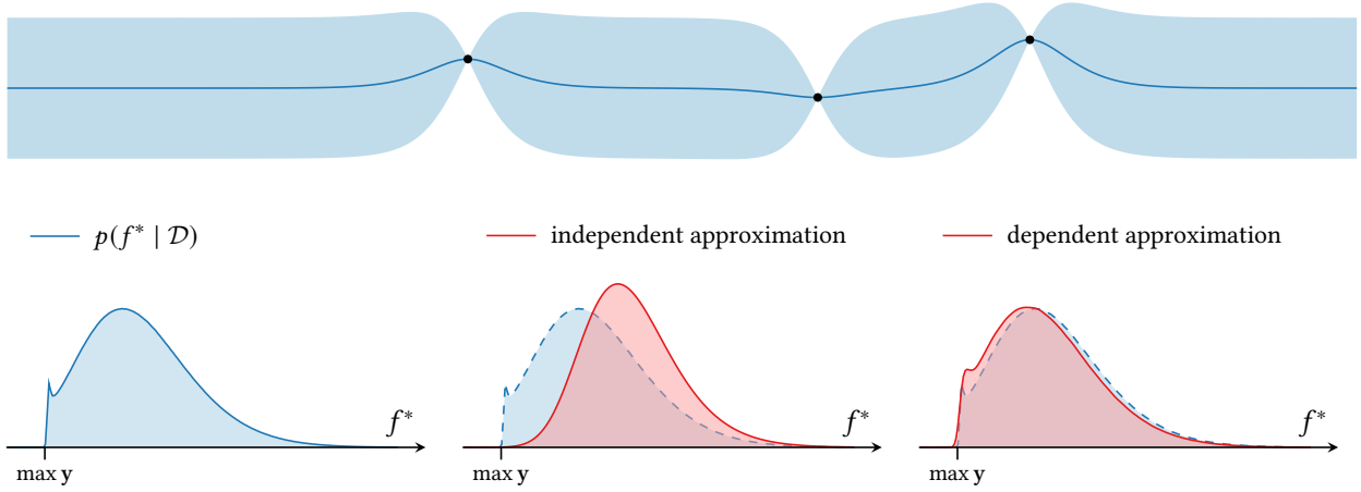
Figure 8.17: Left: the true distribution p(f^* | \mathcal{D}) for our running scenario, estimated using exhaustive sampling. Middle: WANG and JEGELKA's approximation to p(f^* | \mathcal{D}) (8.56) using a grid of 100 equally spaced representer points. Right: an approximation to p(f^* | \mathcal{D}) from sampling the function values at the 100 Thompson samples from Figure 8.11.
