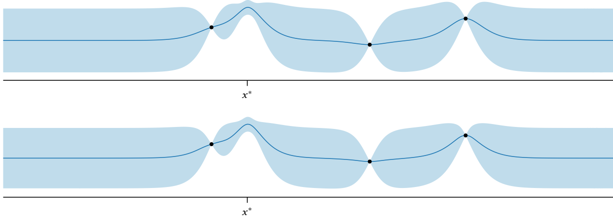
Figure 8.15: Top: the approximate posterior after conditioning on \phi^* exceeding the function values at previously measured locations (8.49). Bottom: the approximate posterior after conditioning on \phi^* dominating elsewhere (8.50).
