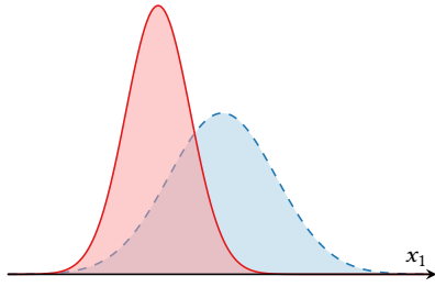
The PDFs of a bivariate Gaussian p(x_1, x_2) (top) and the conditional distribution p(x_1 | x_2) given the value of x_2 marked by the dashed line (bottom) (A.14). The prior marginal distribution p(x_1) is shown for reference; the observation decreased both the mean and standard deviation.
