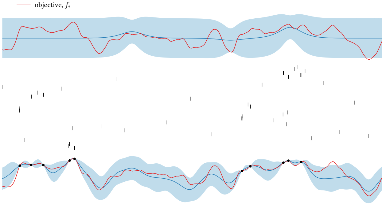
Figure 11.8: A simulation of optimization with the cost-adjusted multifidelity expected improvement starting from the scenario in Figure 11.7. We simulate sequential observations of either the objective or the surrogate, illustrated using the running tick marks. The lighter marks correspond to surrogate observations and the heavier marks correspond to objective observations. The optimum was found after 10 objective observations and 32 surrogate observations. The prior (top) and posterior (bottom) of the objective function conditioned on all observations are also shown.
