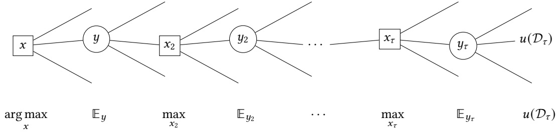
Figure 5.4: The optimal optimization policy as a decision tree. Squares indicate decisions (the choice of each observation), and circles represent expectations with respect to random variables (the outcomes of observations). Only one possible optimization path is shown; dangling edges lead to different futures, and all possibilities are always considered. We maximize the expected terminal utility u(\mathcal{D}_\tau) , recursively assuming optimal future behavior.
