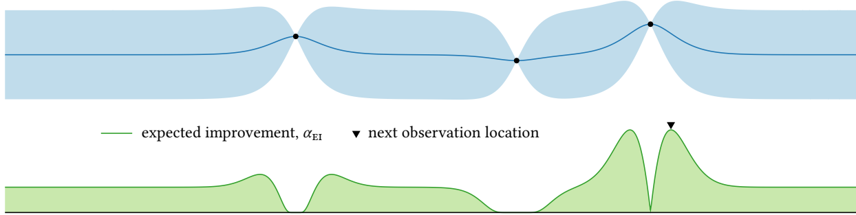
Figure 7.3: The expected improvement acquisition function (7.2) corresponding to our running example.
