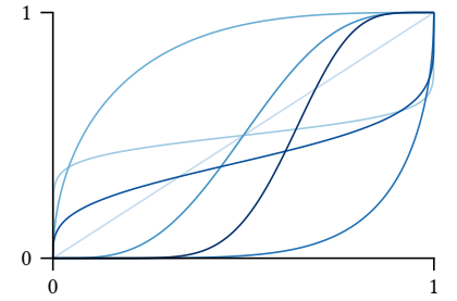
Some examples of beta CDF warping functions (3.28).
