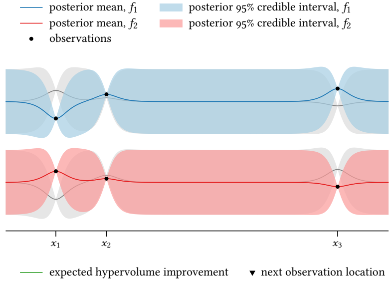
Figure 11.12: The posterior belief about our example objectives from Figure 11.10 given observations at the marked locations. The beliefs are separated vertically (by an arbitrary amount) for clarity, with the belief over the other function shown for reference.
