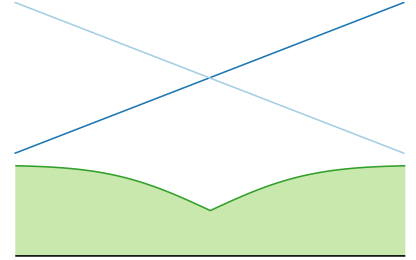
Above: the two possible objectives for our comparison of the \mathbb{E}u and u\mathbb{E} . Below: the expected marginal gain in u\mathbb{E} , which prefers sampling on the boundary to reveal more information regarding the model. The expected marginal gain in \mathbb{E}u is constant.
