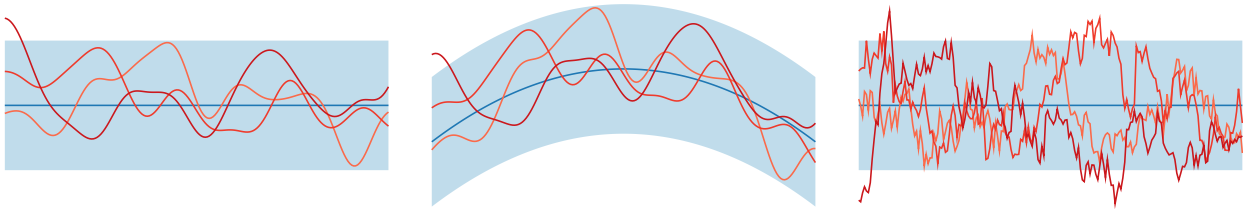
Figure 3.1: The importance of the prior mean function in determining sample path behavior. The models in the first two panels differ in their mean function but share the same covariance function. Sample path behavior is identical up to translation. The model in the third panel features the same mean function as the first panel but a different covariance function. Samples exhibit dramatically different behavior.
