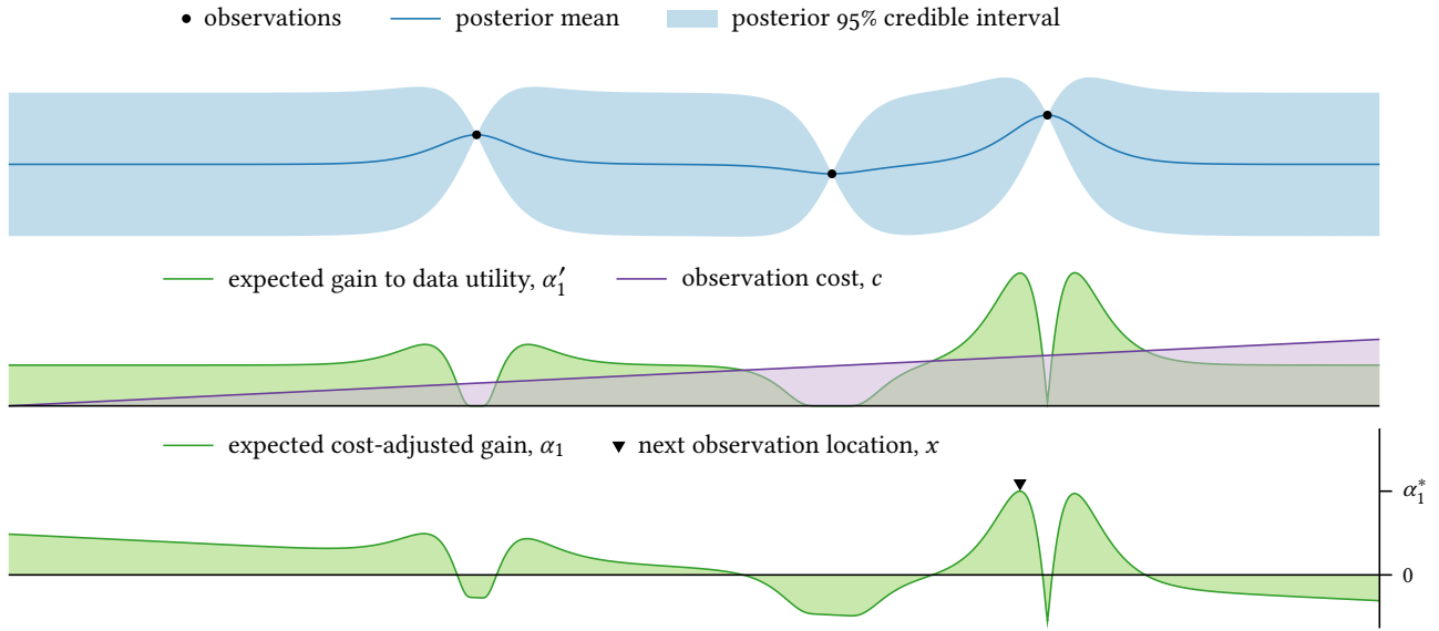
Figure 5.8: Illustration of one-step lookahead with the option to terminate. With a linear utility and additive costs, the expected marginal gain \alpha_1 is the expected marginal gain to the data utility \alpha_1' adjusted for the cost of acquisition c . For some points, the cost-adjusted expected gain is negative, in which case we would prefer immediate termination to observing there. However, continuing with the chosen point is expected to increase the utility of the current data.
