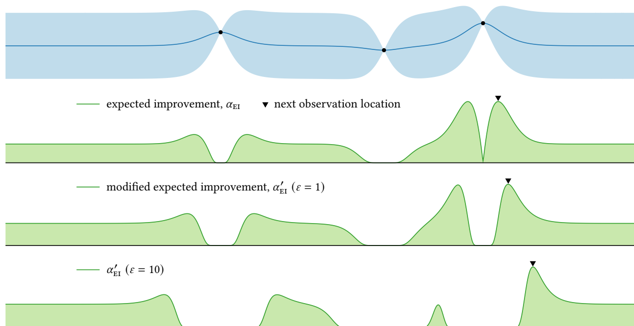
Figure 7.23: The modified expected improvement acquisition function (7.21) for our running example for different values of the target improvement \varepsilon . The target is expressed as a fraction of the range of the posterior mean over the space. Increasing the target improvement leads to increasingly exploratory behavior.
