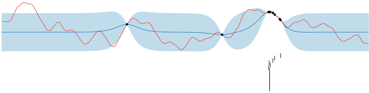
Figure 7.25: The posterior after 15 steps of two-step lookahead for cumulative reward (7.22) on our running example. The tick marks show the points chosen by the policy, progressing from top to bottom. The policy becomes stuck on iteration 7.
