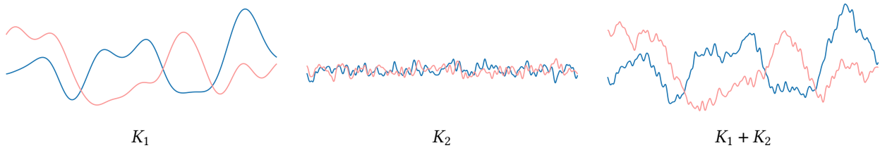
Figure 3.8: Samples from centered Gaussian processes with different covariance functions: (left) a squared exponential covariance, (middle) a squared exponential covariance with smaller output scale and shorter length scale, and (right) the sum of the two. Samples from the process with the sum covariance show smooth variation on two different scales.
