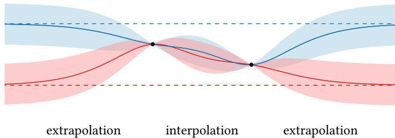
Figure 3.2: The influence of the prior mean on the posterior mean. We show two Gaussian process posteriors differing only in their prior mean functions, shown as dashed lines. In the “interpolatory” region between the observations, the posterior means are mostly determined by the data, but devolve to the respective prior means when extrapolating outside this region.
