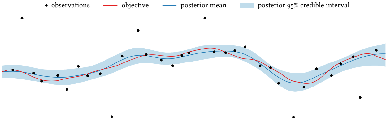
Figure 2.12: Regression with observations corrupted with heavy-tailed noise. The triangular marks indicate observations lying beyond the plotted range. Shown is the posterior distribution of an objective function (along with ground truth) modeling the errors as Student- t distributed with \nu = 4 degrees of freedom. The posterior was approximated from 100 000 Monte Carlo samples. Comparing with the additive Gaussian noise model from Figure 2.10, this model effectively ignores the outliers and the fit is excellent.
