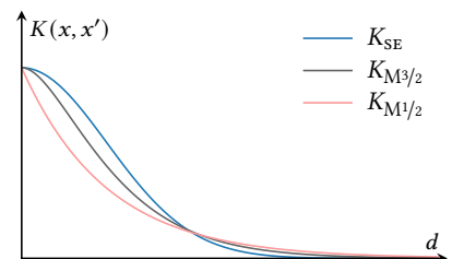
Some members of the Matérn family and the squared exponential covariance as a function of the distance between inputs. All decay to zero correlation as distance increases.
