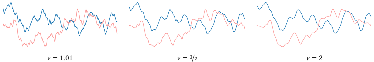
Figure 10.3: Sample paths from a centered GP with Matérn covariance with smoothness parameter \nu ranging from just over 1 (left) to 2 (right). The random seed is shared so that corresponding paths are comparable across the panels. All samples are once differentiable, but some are smoother than others.
