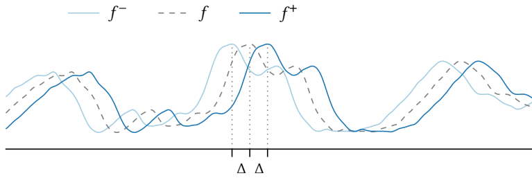
Figure 10.4: A sketch of SCARLETT’s proof strategy. Given access to a reference function f , which of its translations by \Delta , f^- or f^+ is the objective function?
