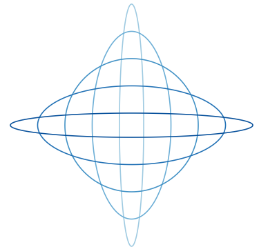
Possible surfaces of equal covariance with the center when combining separate dilation of each axis with an isotropic covariance.
