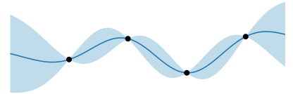
The first of many “sausage plots” to come.
