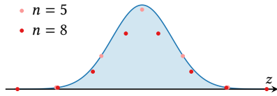
Gauss–Hermite nodes/weights for n \in \{5, 8\} .
