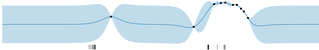
Figure 7.12: The points maximizing probability of improvement using the 27 improvement thresholds proposed by JONES, beginning with the posterior from Figure 7.10 after 10 total observations have been obtained. The tick marks show the chosen points and cluster together in four regions representing different tradeoffs between exploration and exploitation.
