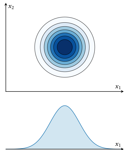
A bivariate Gaussian PDF p(\mathbf{x}_1, \mathbf{x}_2) (top) and the Gaussian marginal p(x_1) (bottom) (A.13).
