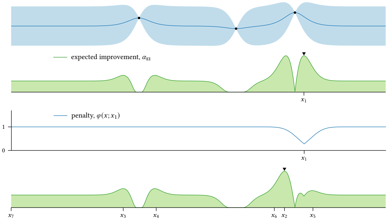
Figure 11.5: Batch construction via local penalization of the expected improvement acquisition function (7.2). We select the first point by maximizing the expected improvement, after which the acquisition function is multiplied by a penalty factor discouraging future batch members in that area. We then maximize the updated acquisition function, penalize, and repeat as desired. The bottom panel indicates the locations of several further points selected in this manner.
