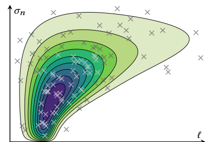
The 100 hyperparameter samples used to produce Figure 4.6.
