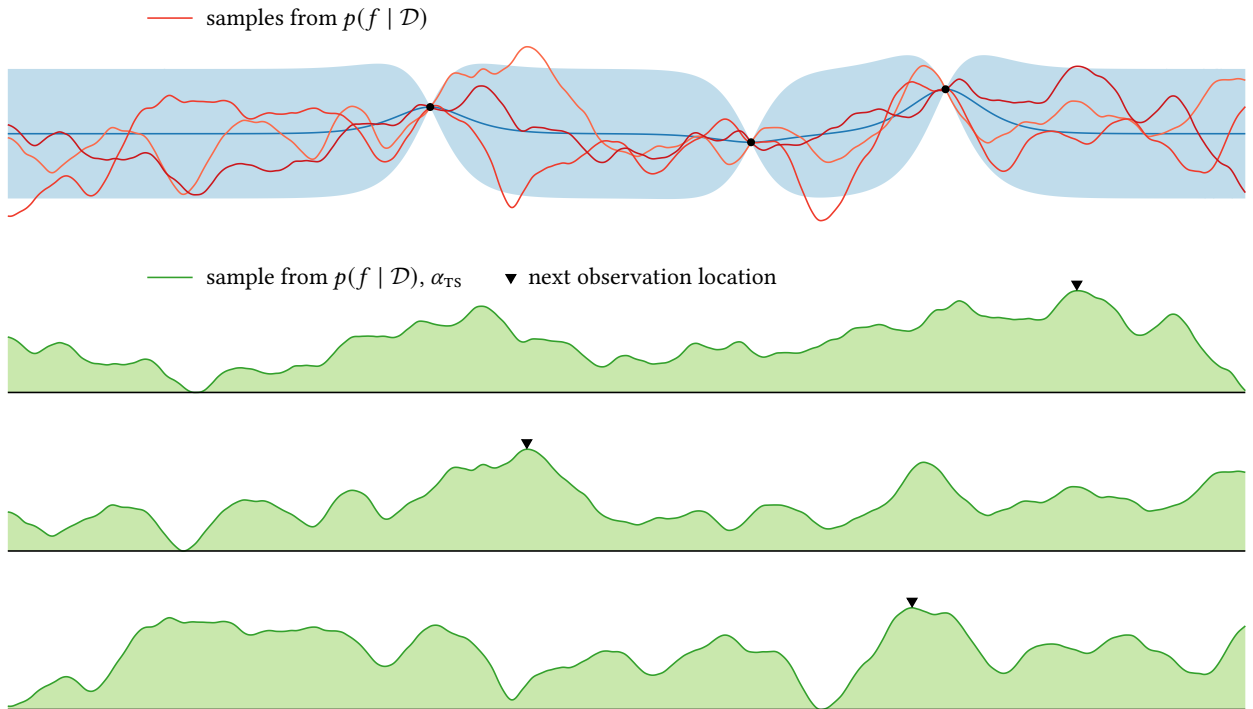
Figure 7.19: An illustration of Thompson sampling for our example optimization scenario. At the top, we show the objective function posterior p(f \mid \mathcal{D}) and three samples from this belief. Thompson sampling selects the next observation location by maximizing one of these samples. In the bottom three panels we show three possible outcomes of this process, corresponding to each of the sampled objective functions illustrated in the top panel.
