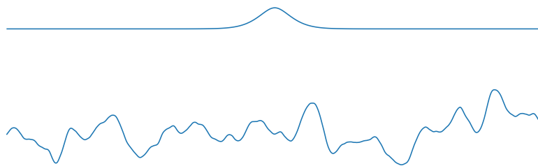
Figure 10.6: The problem with estimating hyperparameters. Above: a function in the RKHS for the \nu = 5/2 Matérn covariance with unit norm. Below: a sample path from a Gaussian process with the same covariance. Unless we're lucky, we may never find the "hump" in the former function and thus may never build a reasonable belief regarding the objective.
