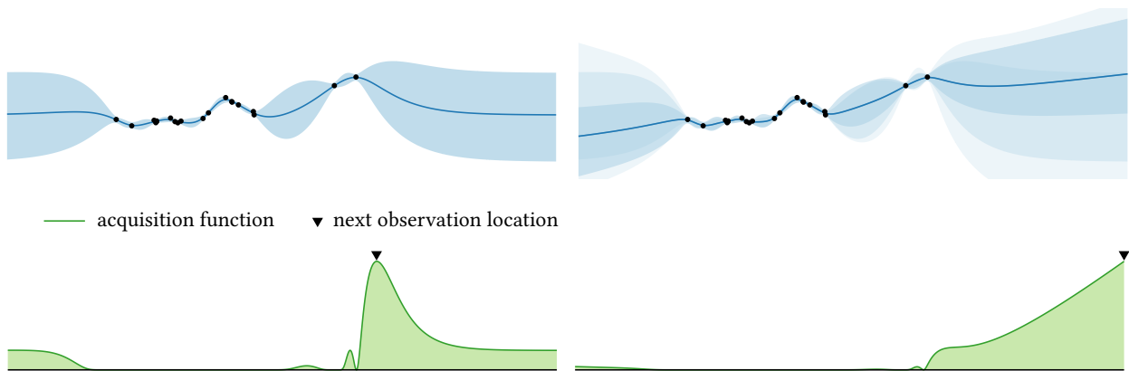
Figure 4.12: Optimization policies built from the MAP M_5 model (left) and the structure-marginal posterior (right). The M_5 model chooses to exploit near the local optimum, but the structure-marginal model is aware of the underlying linear trend and chooses to explore the right-hand side as a result.
