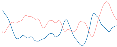
Sample paths of a stationary Gaussian process with Matérn \nu = 5/2 covariance (3.14) show more regularity than arbitrary continuous functions.
