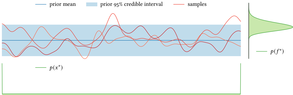
Figure 6.3: The objective function prior used throughout our utility function comparison. Marginal beliefs of function values are shown, as well as the induced beliefs over the location of the global optimum, p(x^*) , and the value of the global optimum, p(f^*) . Note that there is a significant probability that the global optimum is achieved on the boundary of the domain, reflected by large point masses.
