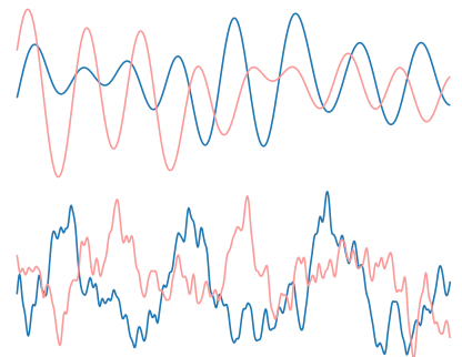
Samples from centered Gaussian processes with two realizations of a Gaussian spectral mixture covariance function, offering a glimpse into the flexibility of this class.
