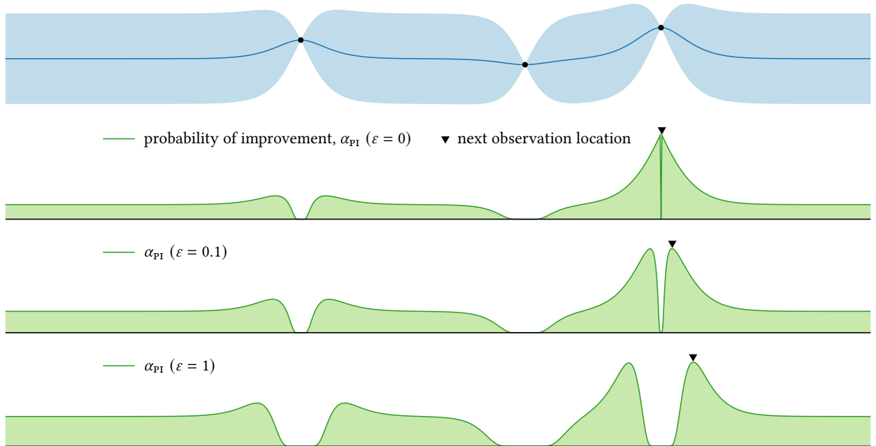
Figure 7.9: The probability of improvement acquisition function (7.5) corresponding to our running example for different values of the target improvement \varepsilon . The target is expressed as a fraction of the range of the posterior mean over the space. Increasing the target improvement leads to increasingly exploratory behavior.
